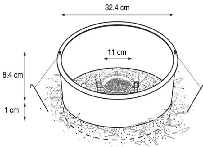
FIGURE 2 | ILLUSTRATION DESIGN FOR THE CHAMBER INSERTED INTO THE SOIL, WITH CERAMIC CUPS CONTAINING SODA LIME ON WIRE STAND. 8.4 CM IS THE HEIGHT OF THE CHAMBER ABOVE THE SOIL SURFACE - THIS SPACE GIVES THE HEAD SPACE OF THE CHAMBER THAT ALLOWS FOR THE EFFLUX OF CARBON DIOXIDE. 1 CM IS THE DEPTH TO WHICH THE CHAMBER IS INSERTED INTO THE SOIL.
